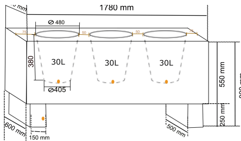
EXTENDO-A — Weight: 45 kg | Capacity: 3X 30 L
