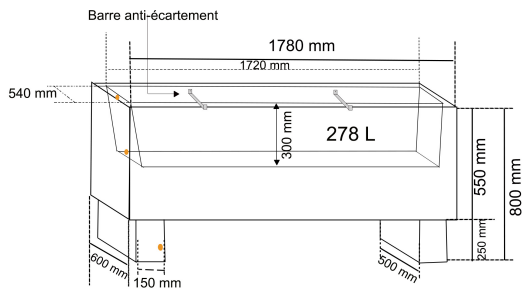
EXTENDO — Weight: 45 kg | Capacity: 278 L
